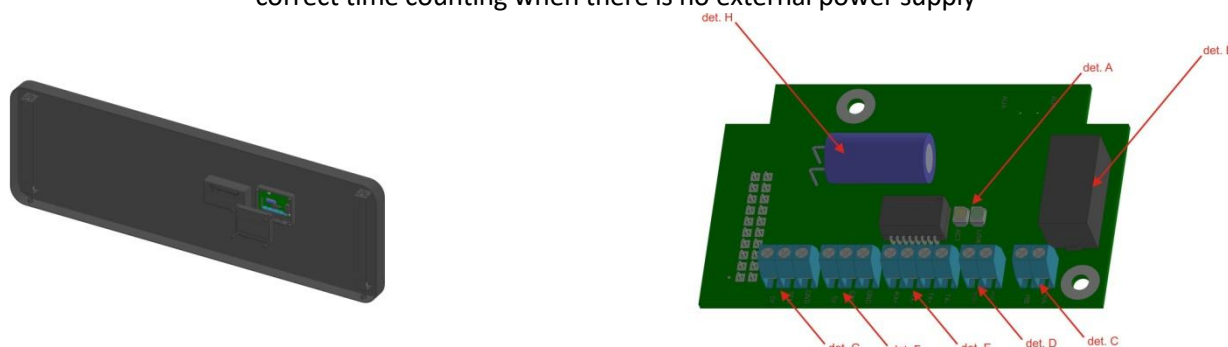
det. A signal LEDs; det. B – relay; det. C – relay connector; det. D – PoE output ; det. E – LAN connector; det. F – GPS connector; det. G – temperature probe connector; det. H – supercapacitor
