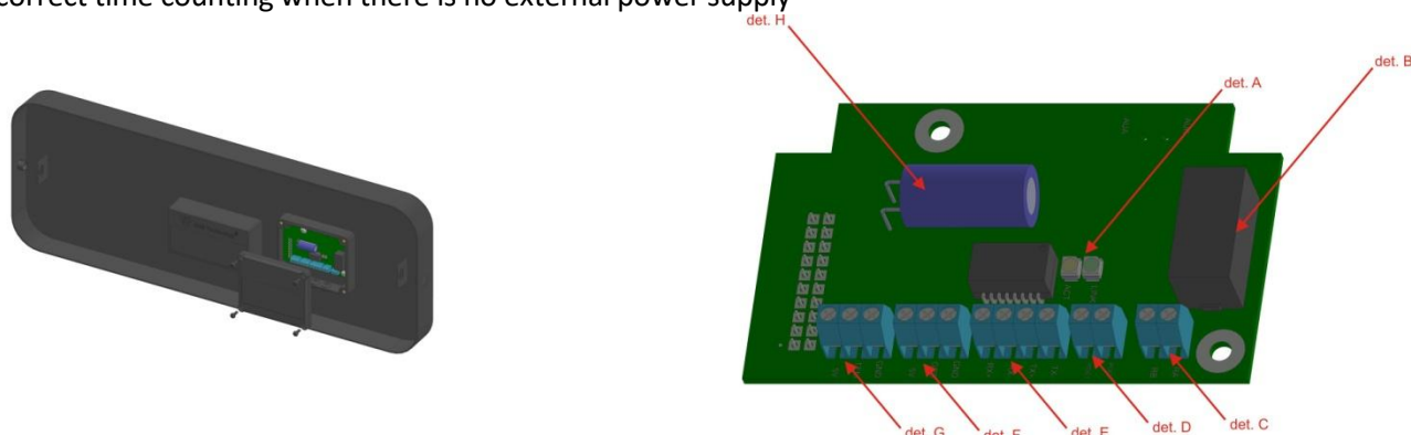
det. A signal LEDs; det. B – relay; det. C – relay connector; det. D – PoE output ; det. E – LAN connector; det. F – GPS connector; det. G – temperature probe connector; det. H – supercapacitor
